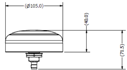
GNSS-L125-40TNC
